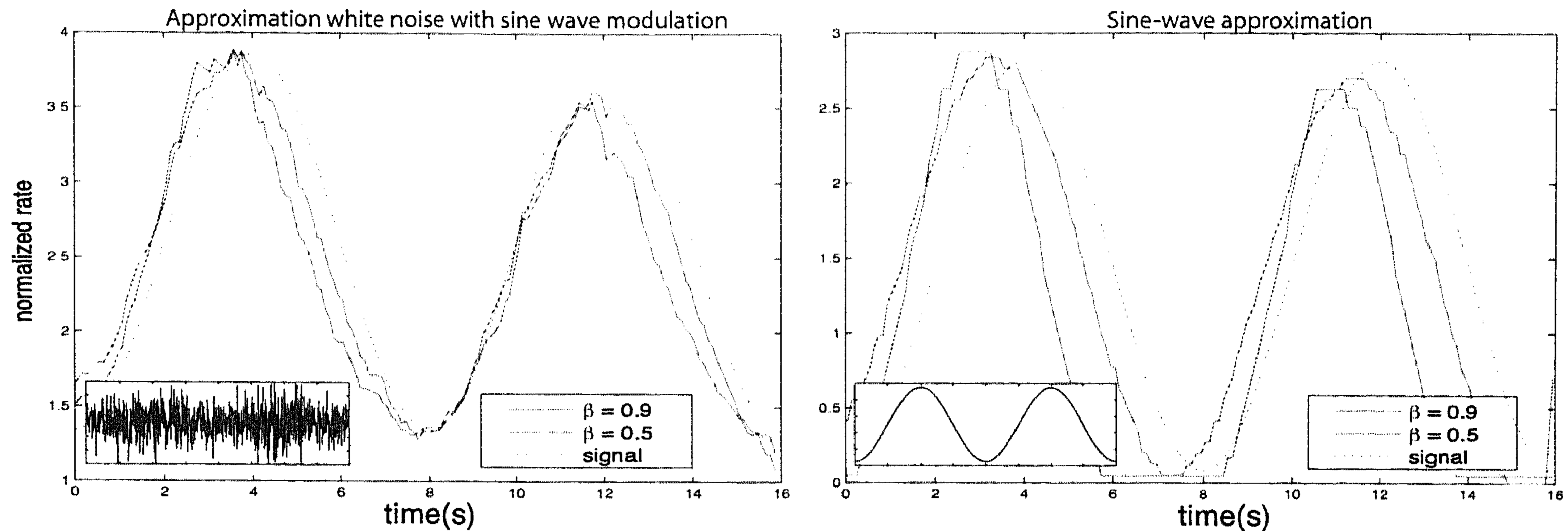
Fig. 4. Sinewave phase-lead. Left: when encoding sine-wave modulated white noise (inset); right: encoding the sine-wave signal itself (inset). Average firing rate is computed over 100ms, and normalized to match the sine-wave kernel.
