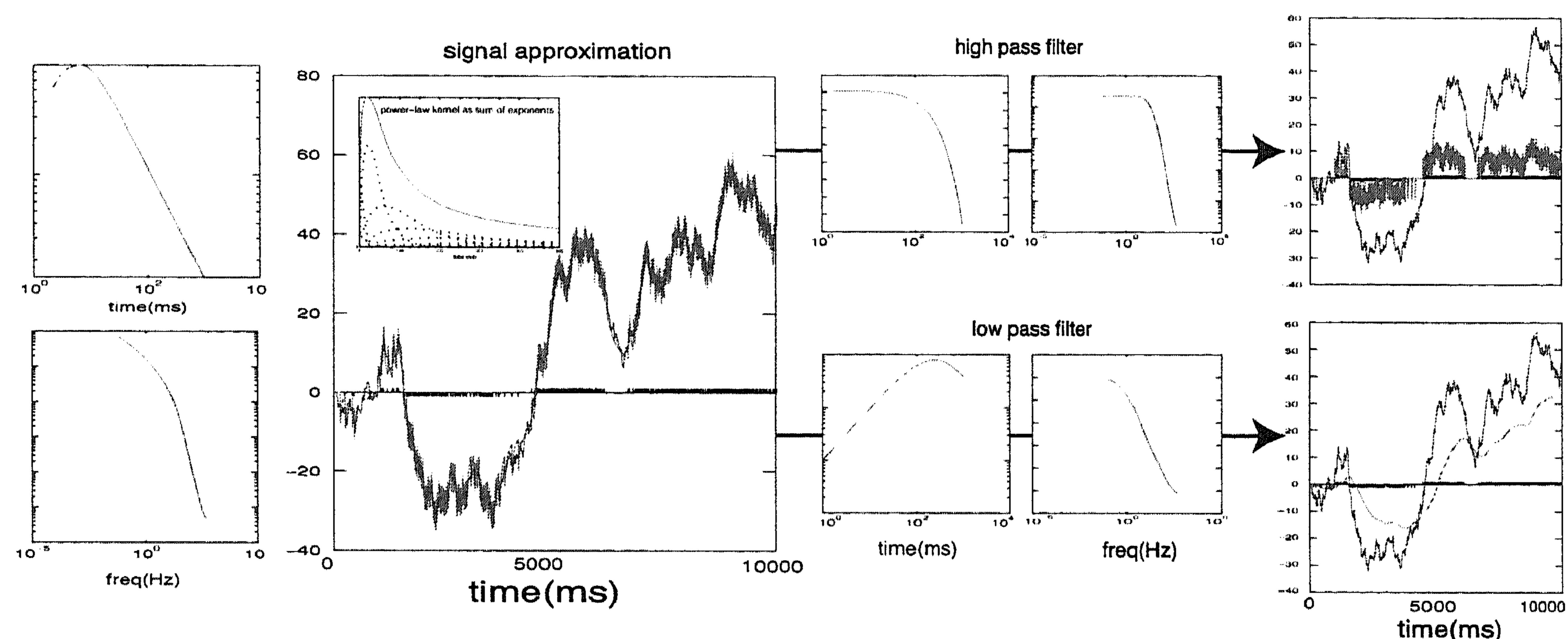
Fig. 5. Illustration of frequency filtering with modified decoding kernels. The square boxes show the respective kernels in both time and frequency space. See text for further explanation.
