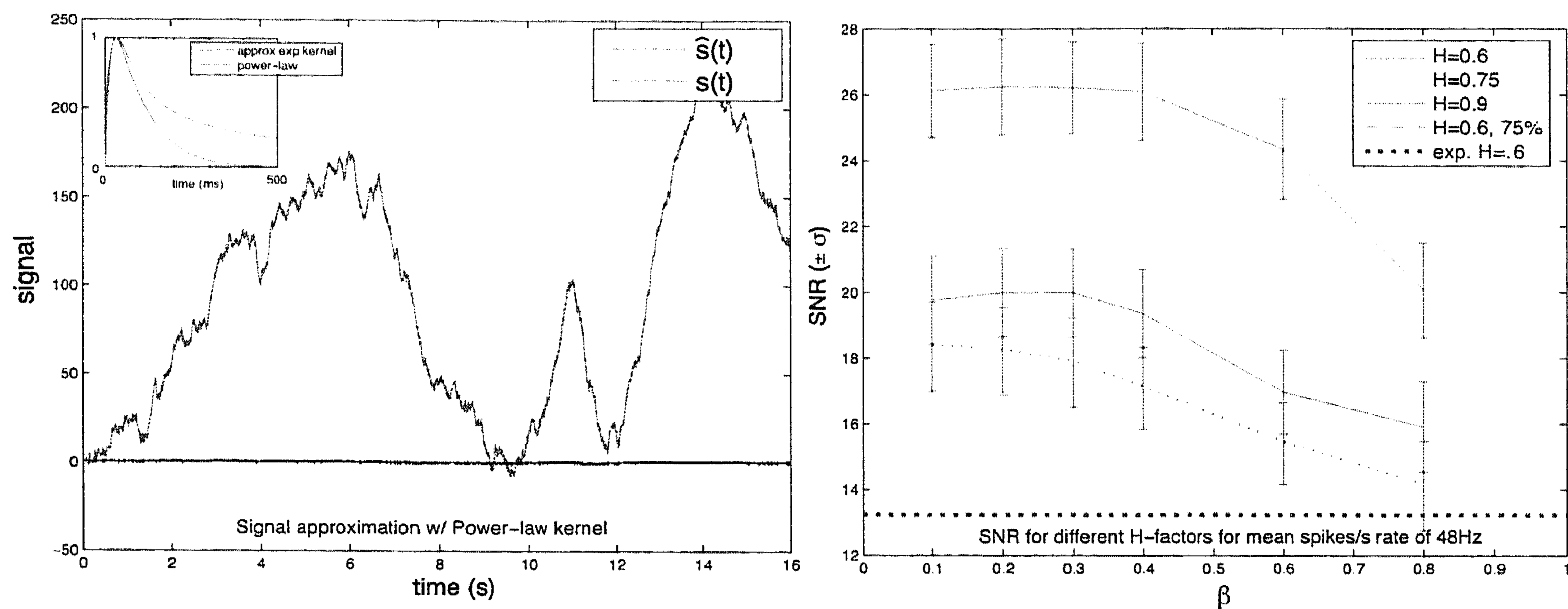
Fig. 3. Left: example of encoding of fBm signal with power-law kernels. Using an exponentially decaying kernel (inset) required 1398 spikes vs. 618 for the power-law kernel ( k = 50 ), for the same SNR. Right: SNR for various \beta power-law exponents using a fixed number of spikes (48Hz), with curves for different H -parameters, each curve averaged over five 16s signals. The dashed blue curve plots the H = 0.6 curve, using less spikes (36Hz); the flat bottom dotted line shows the average performance of the non-power-law exponentially decaying kernel, also for H = 0.6 .
