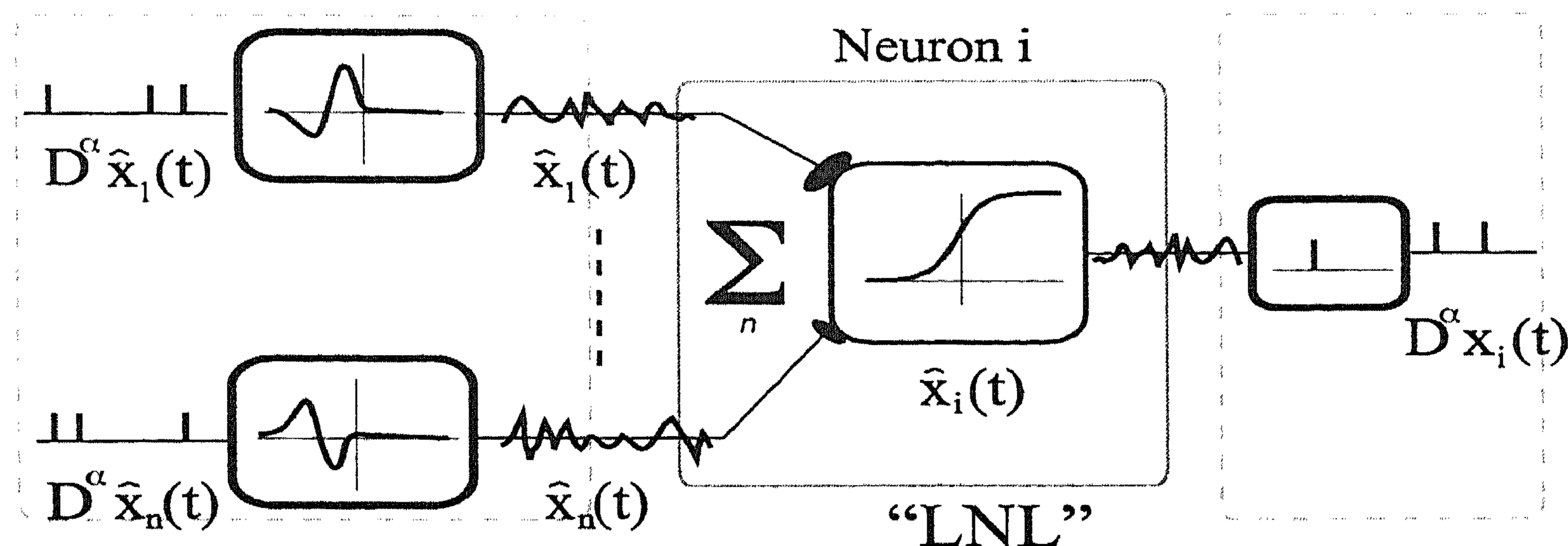
Fig. 1. Linear-Non-Linear filter, with spike-decoding front-end and spike-encoding back-end.
